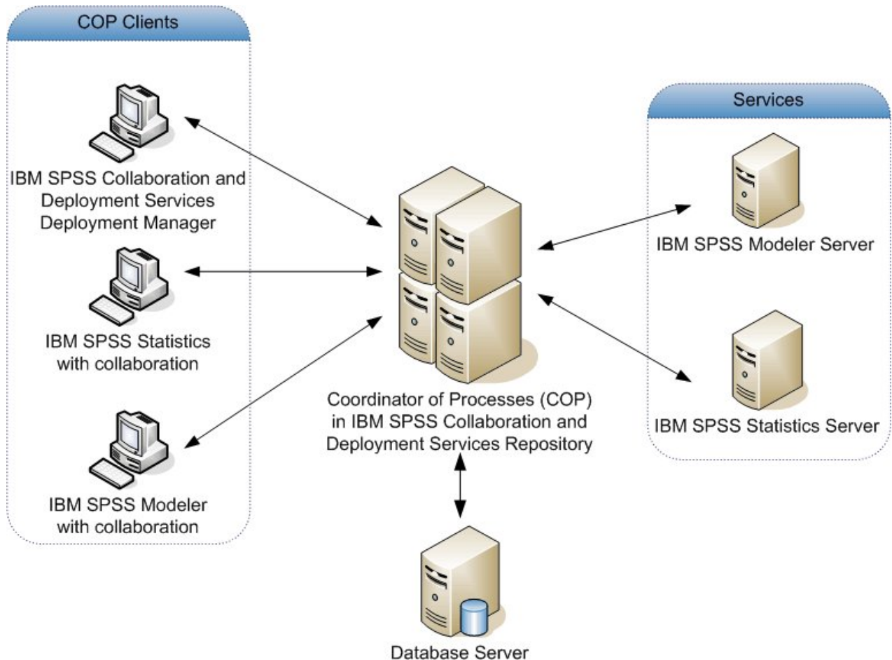
Figure 5. Coordinator of Processes Architecture
